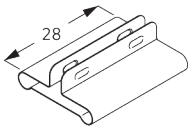
SG 7002 Profile protector
