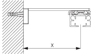
Square Smart Fix SG 11211 - SG 11215 and clamp SG 3004:
