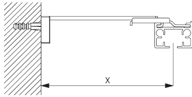
Square Smart Fix SG 11210 - SG 11215 and bracket SG 3041:
