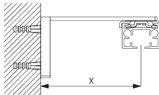
Smart Fix SG 11201 - SG 11205 and clamp SG 3004:
