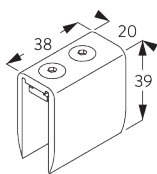
SG 6610 Wall support
