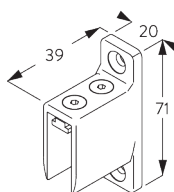
SG 6614 Wall bracket, metal
