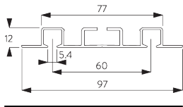
SG 6244p Profile
