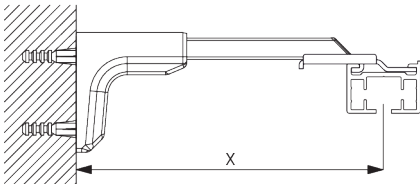
Universal Smart Fix SG 11154 - SG 11156 and bracket SG 3041: Screw SG 10407 (M4x10) needed.
