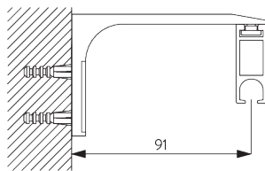
Screw SG 6784 (M4x8) needed.
