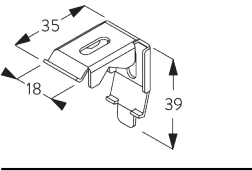
SG 2302 Bracket
