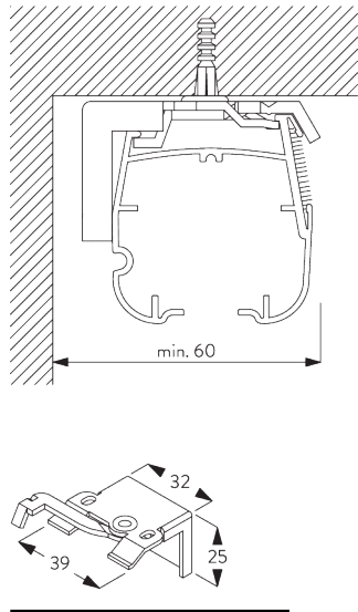
SG 2346 Bracket
