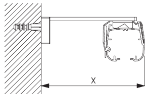
Square Smart Fix SG 11210 - SG 11215 and bracket SG 2302: Screw SG 10395 (M4x6) needed.
