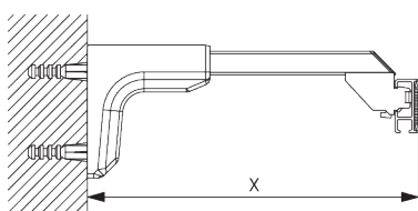
Universal Smart Fix SG 11154 - SG 11156: Screw SG 10277 (M4x12) needed.
