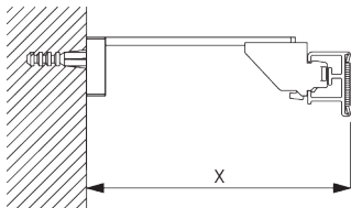
Square Smart Fix SG 11210 - SG 11215 and bracket SG 3603: Screw SG 10492 (M4x8) needed.
