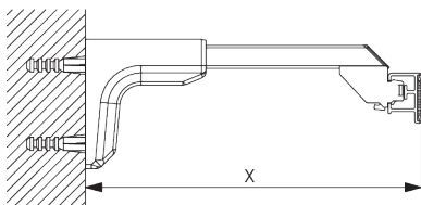
Universal Smart Fix 11154-11156 and bracket SG 3603: Screw SG 10277 (M4x12) needed.
