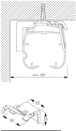
SG 2346 Bracket
