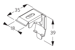
SG 2302 Bracket
