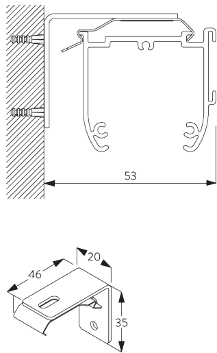
SG 2343 Bracket 46 mm
