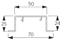
SG 2615 Recess profile
