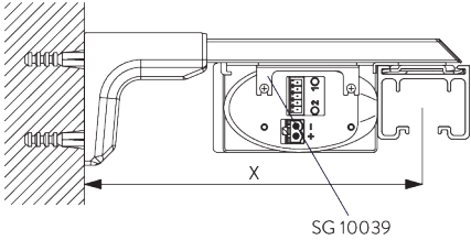
Universal Smart Fix SG 11156 and clamp SG 3033 / SG 3044 Screw SG 11158 (M4x12) needed.
