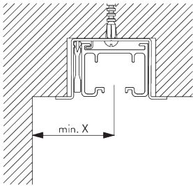
Recess profile SG 2932 can not be bent! Larger recess for motor is necessary! One wedge SG 2941 per fixing point. For detailed recess fitting, visit the Silent Gliss website.
