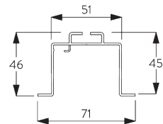
SG 2948 Recess profile
