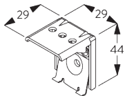
SG 8302 Bracket
