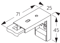
SG 8920 Bracket
